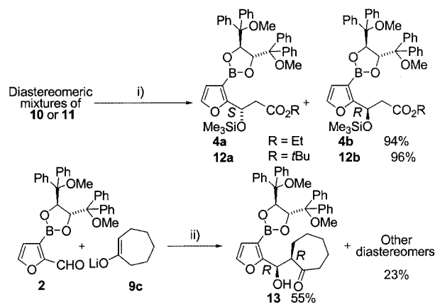
Scheme 2. i) \text{Me}_3\text{SiCl} , imidazole, THF, room temp., 3 h; ii) \text{Et}_2\text{O} , -78^\circ\text{C} to room temp., 14 h
