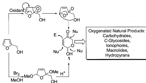
Figure 1. Mechanism for furyl alcohol rearrangement to hydroxypyranone
