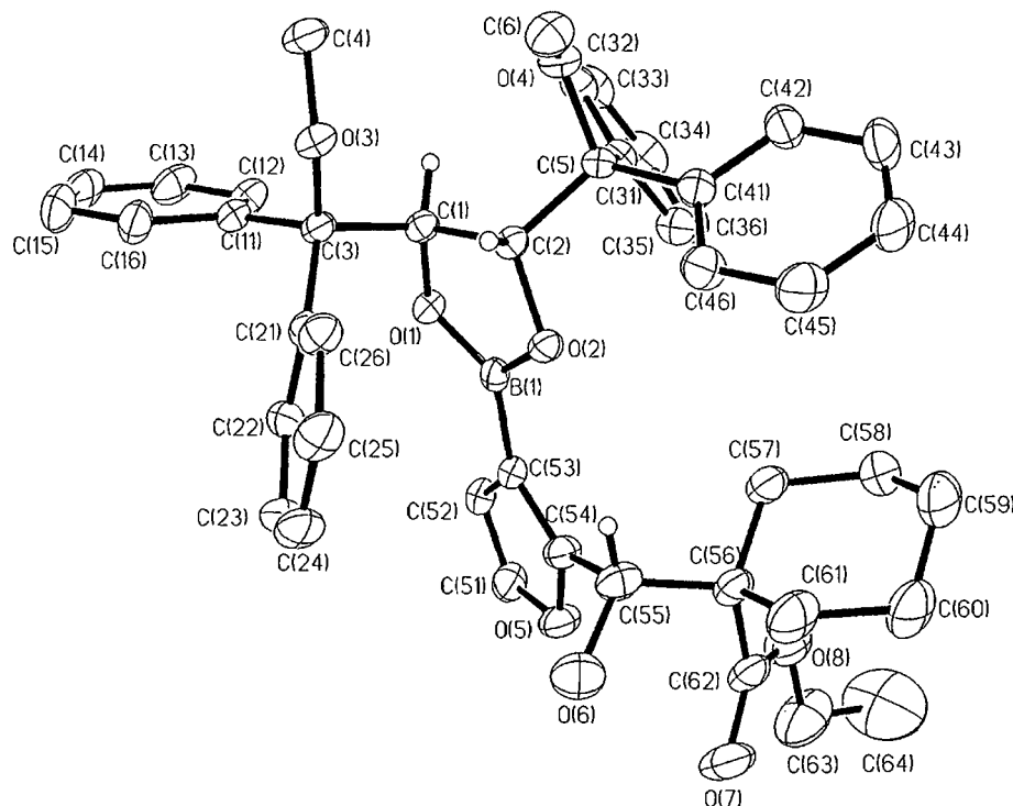
Figure 4. X-ray crystal structure of 8a
