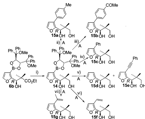
Scheme 3. i) DIBAL-H, THF, 0 °C, 2 h, 94%; ii) iodotoluene, 84%; iii) 4-iodoacetophenone, 95%; iv) iodobenzene, 89%; v) 1-iodo-3-phenylacetylene, 15d , 42%, 15e , 38%; vi) vinyl bromide, 75%; vii) 2-bromopropene, 70%; A: Pd(PPh 3 ) 4 , Ba(OH) 2 , DME/H 2 O (4:1), reflux, 1 h
