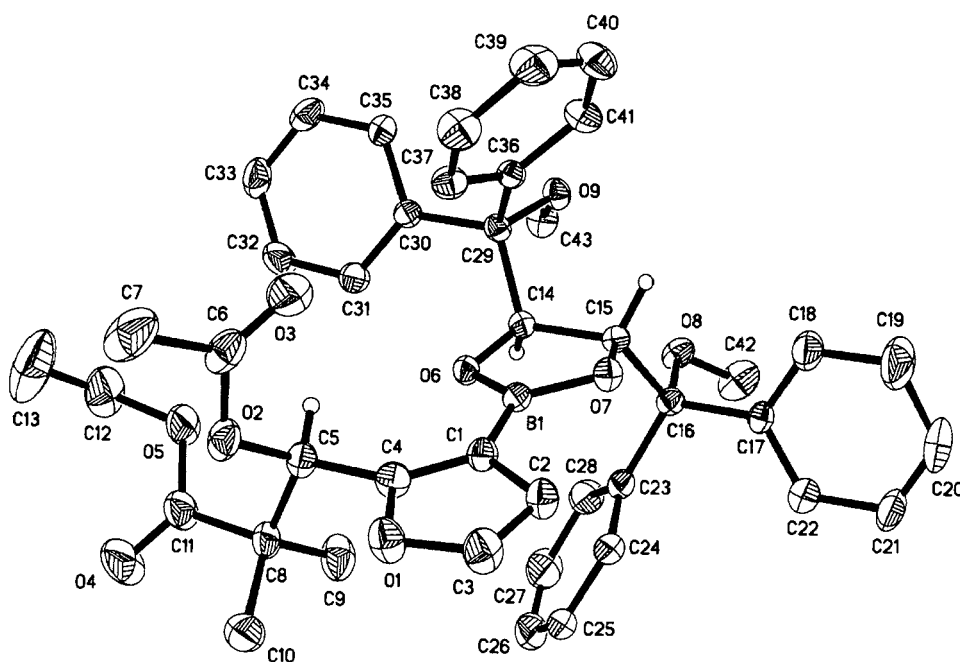
Figure 3. X-ray crystal structure of 7
