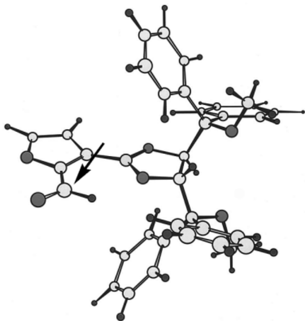
Figure 5. The arrow indicates the more favorable Re -face attack of aldehyde 2
