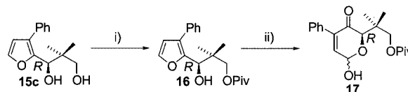
Scheme 4. i) PivCl, pyridine, room temp., 1 h, 89%; ii) NBS, EtOAc, reflux, 4 h, 82%
