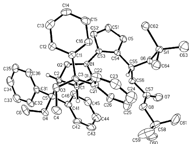
Figure 6. X-ray crystal structure of 12b
