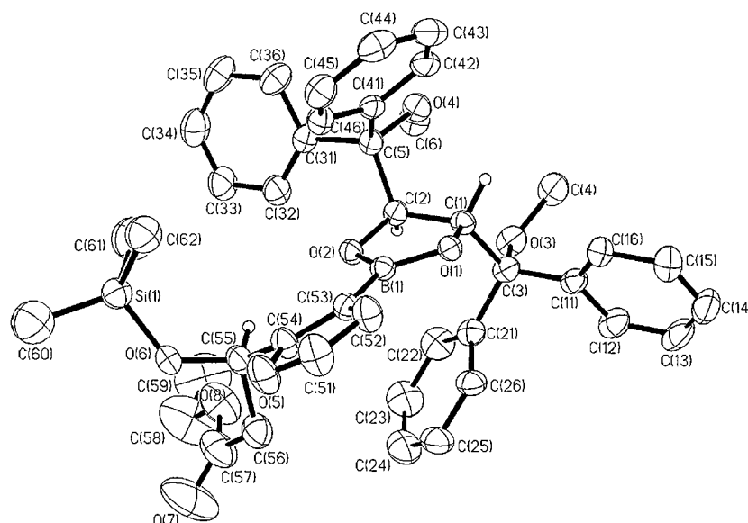
Figure 2. X-ray crystal structure of 4b
