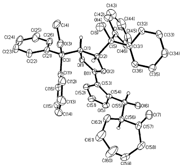
Figure 7. X-ray crystal structure of 13
